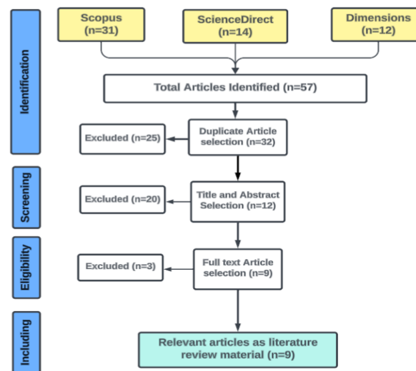
Figure 1. PRISMA diagram.
