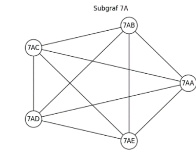
Figure 9. Subgraph S_7
