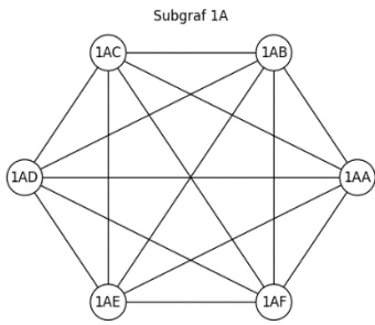
Figure 3. Subgraph S_1
