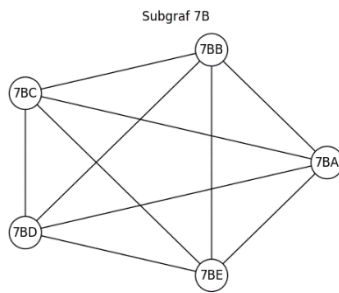
Figure 10. Subgraph S_8
