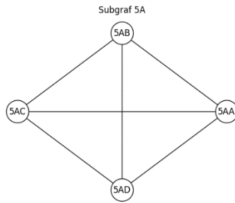
Figure 7. Subgraph S_5
