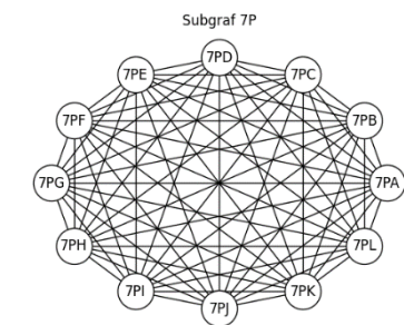
Figure 12. Subgraph S_{10}
