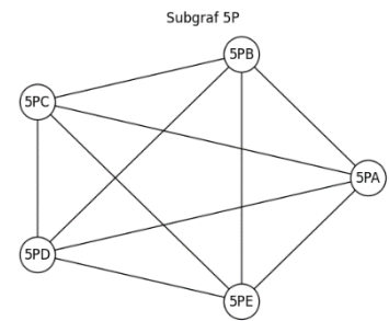
Figure 11. Subgraph S_9
