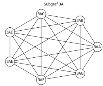
Figure 5. Subgraph S_3
