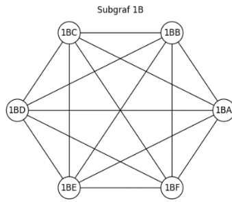
Figure 4. Subgraph S_2
