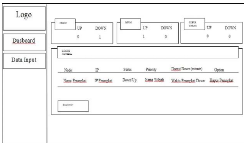
Gambar 2. Login cacti
